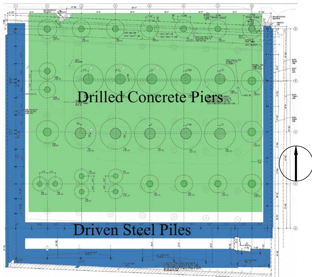
Fig. 6: Foundation plan
